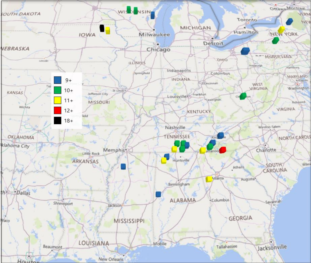
Figure 3 GHCN STATIONS WITH AUGUST MONTHLY PRECIPITATION RECORDS DURING AUGUST 2021 VERSUS AUGUSTS IN THE PERIOD 1960-2021 WHICH EXCEEDED NINE INCHES OF PRECIPITATION FOR THE MONTH
