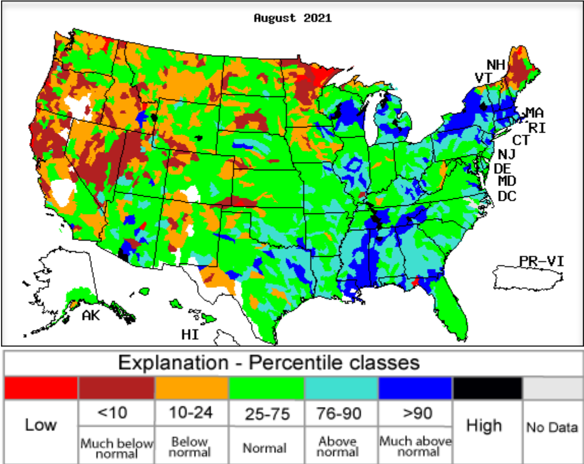
Figure 4 UNITED STATES GEOLOGICAL SURVEY (USGS) STREAMFLOW IN AUGUST 2021 VS HISTORICAL DATA PERCENTILE CLASSES USING STREAMGAGES WITH AT LEAST 30 YEARS OF DATA
