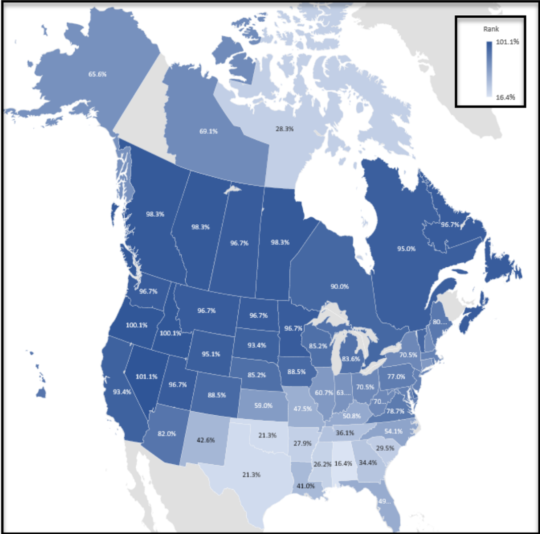
Figure 1 GHCN PERCENTILE RANKINGS OF 2021 DURING 1960-2021 FOR U.S. STATES AND CANADIAN PROVINCES DAILY MAXIMUM TEMPERATURE (TMAX) OVER THE METEOROLOGICAL SUMMER PERIOD (JUNE, JULY, AUGUST)
