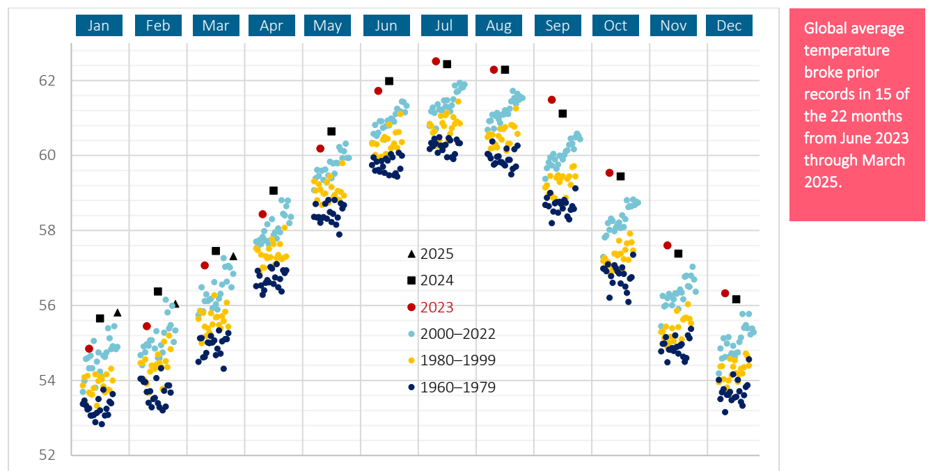
Figure 3 GLOBAL AVERAGE AIR TEMPERATURE (F) BY MONTH
